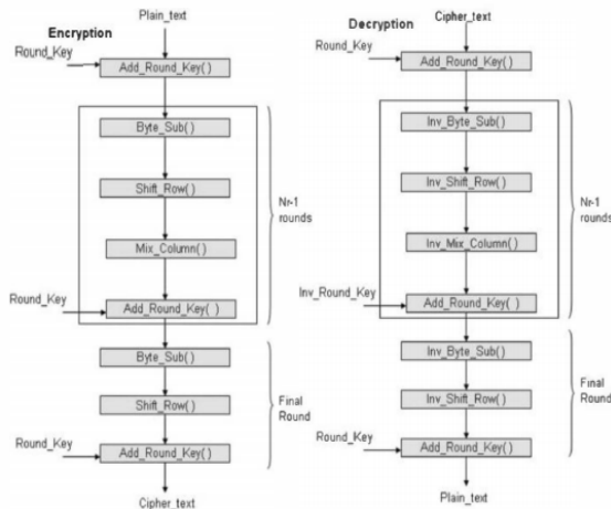
Fig1: AES algorithm
