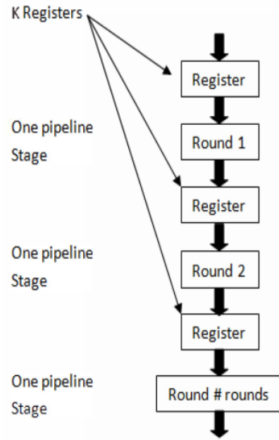
Fig2 pipelined AES
